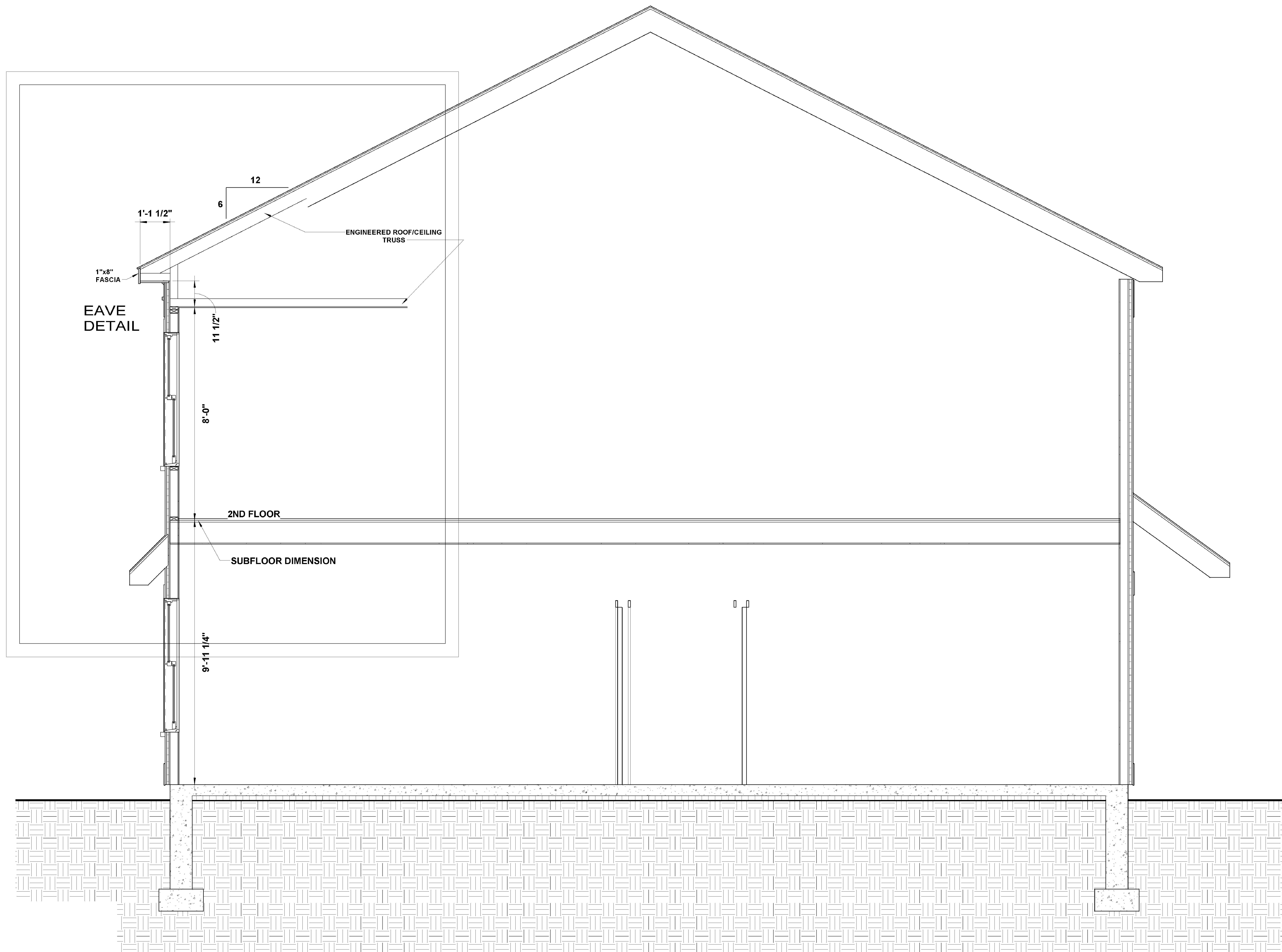
1 COMPOSITE SECTION 1 1/2" = 1'-0"
